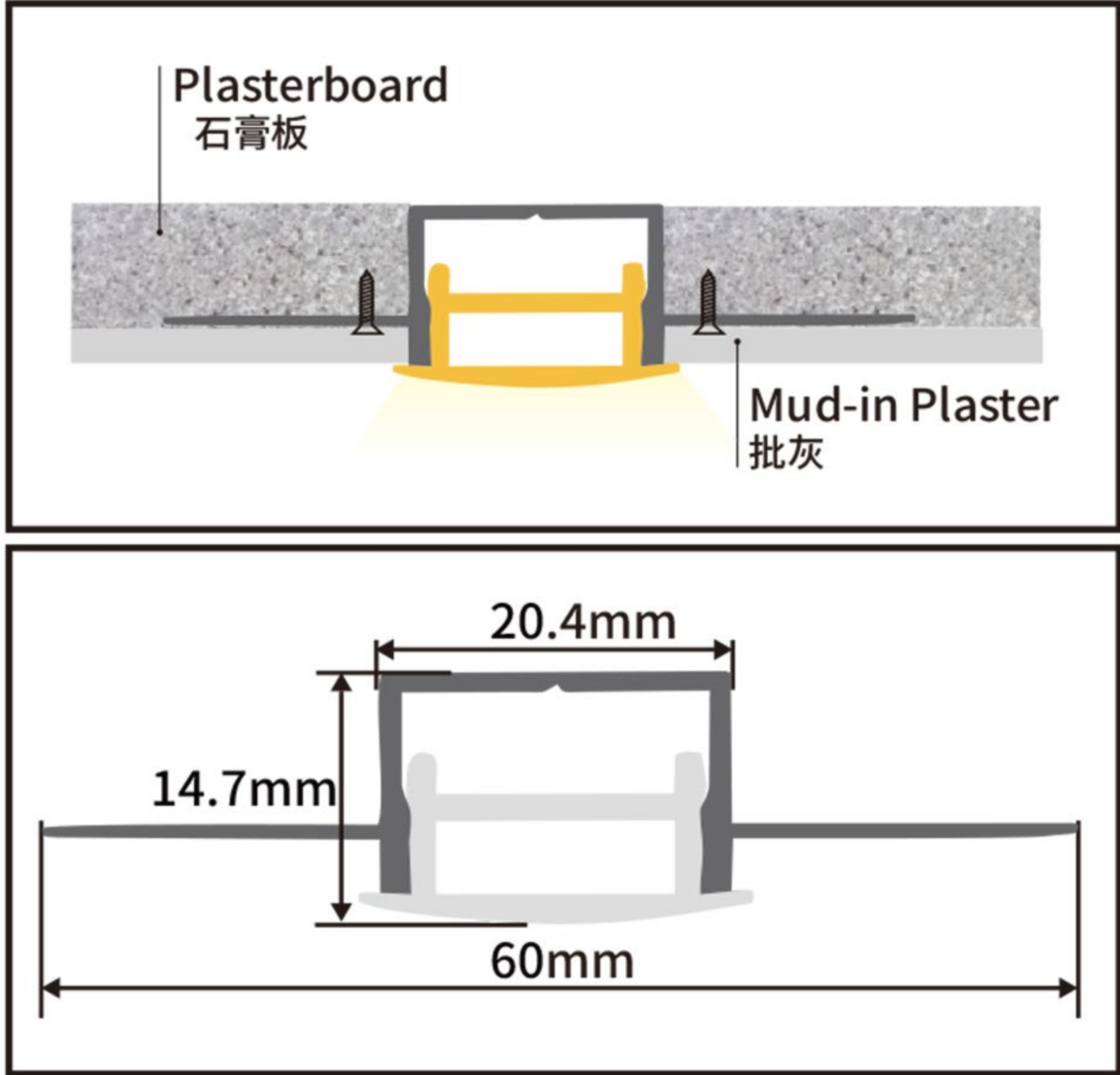
LFAPSL-DW-60X14.7X20.4
