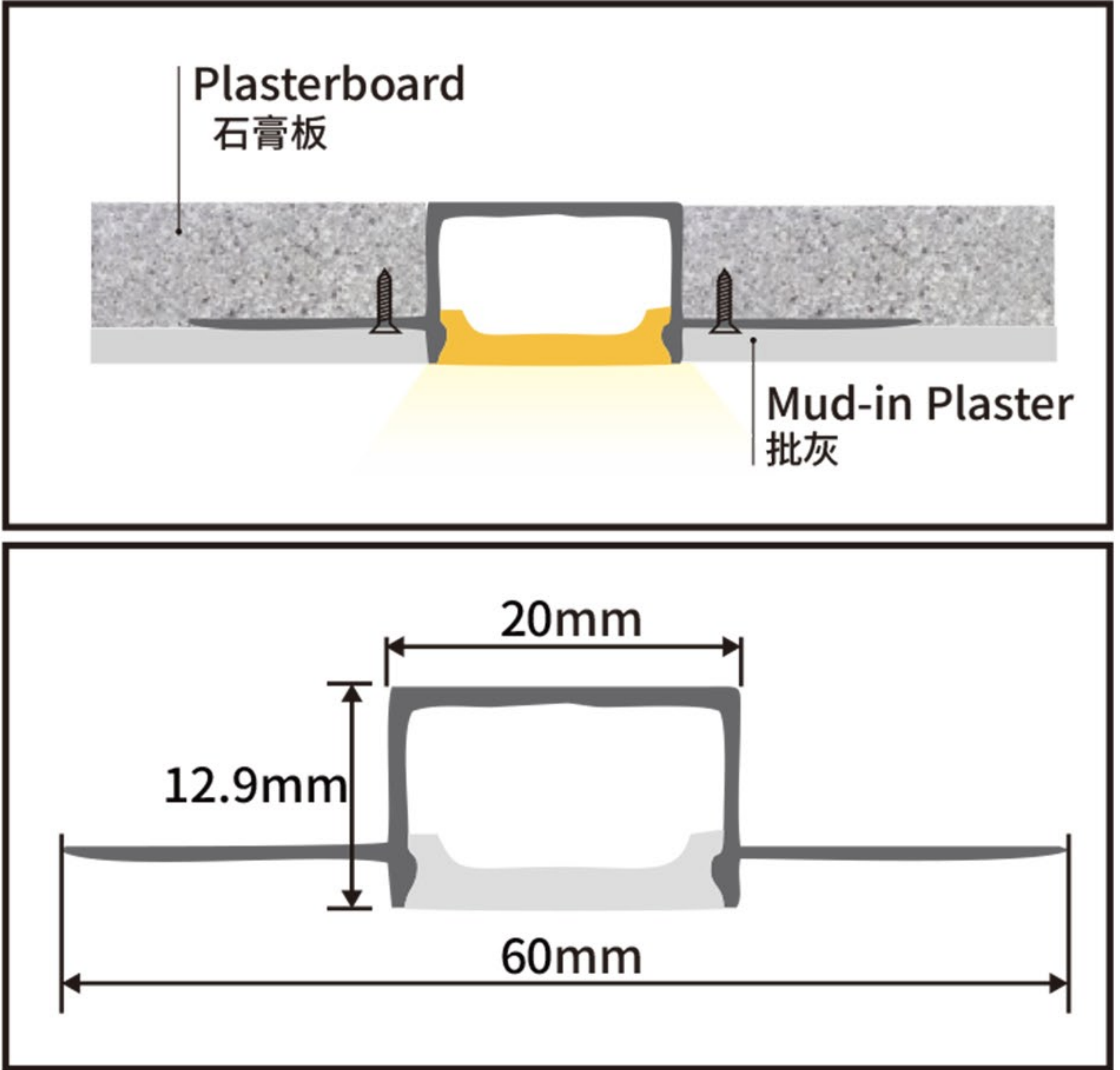
LFAPSL-DW-60X12.9X20
