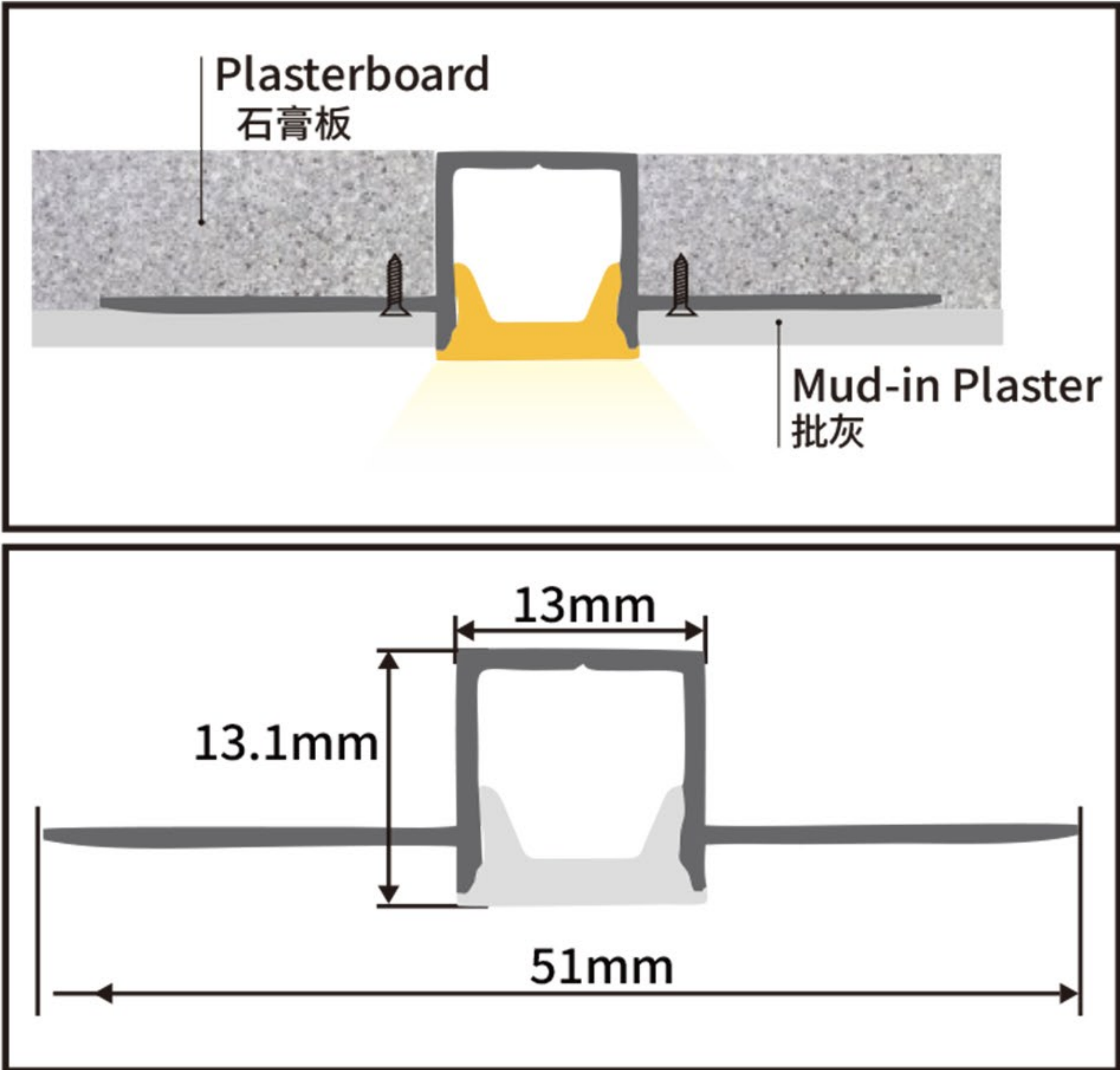
LFAPSL-DW-51X13.1X13
