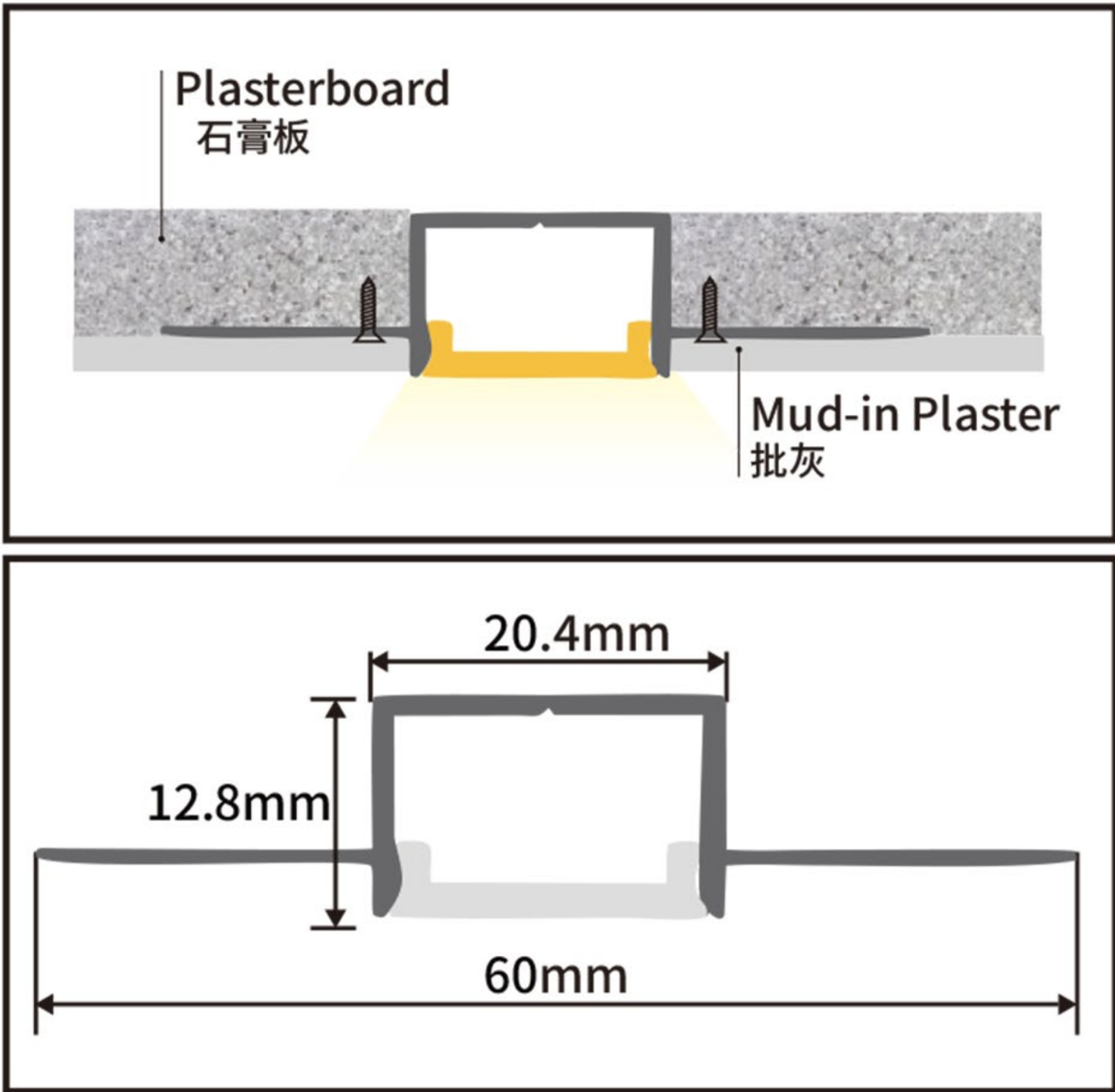
LFAPSL-DW-60X12.8X20.4
