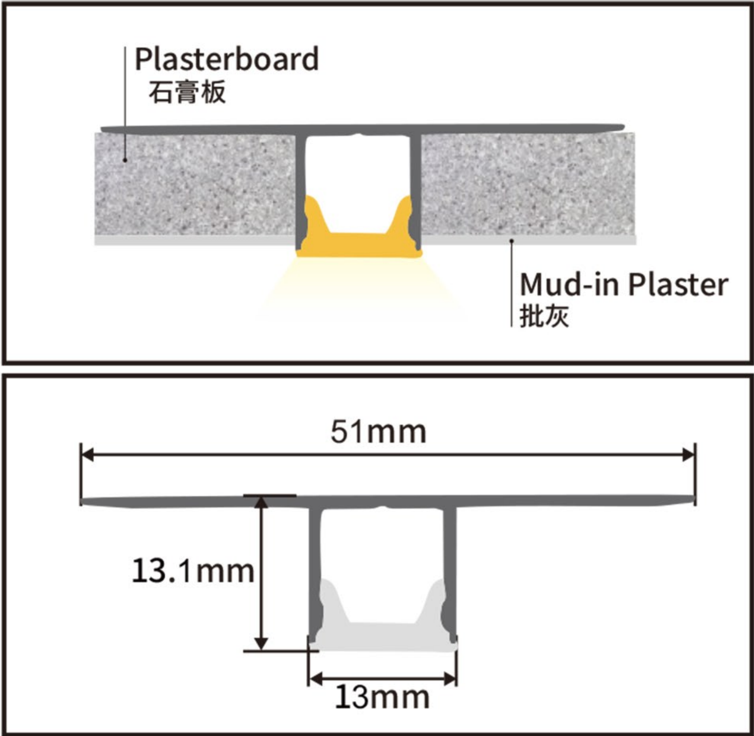
LFAPSLS-DW-51X13.1X13
