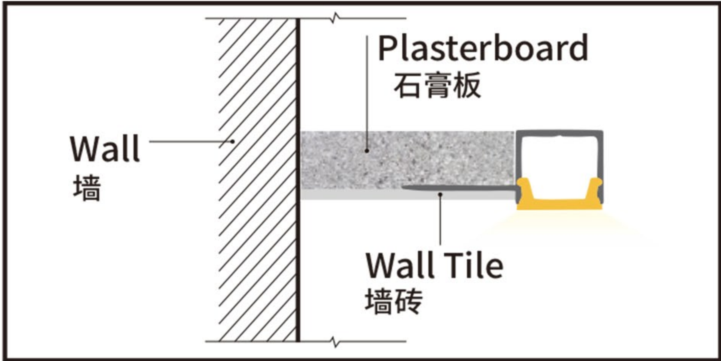
LFAPSL-SWL-34.4X14X15
