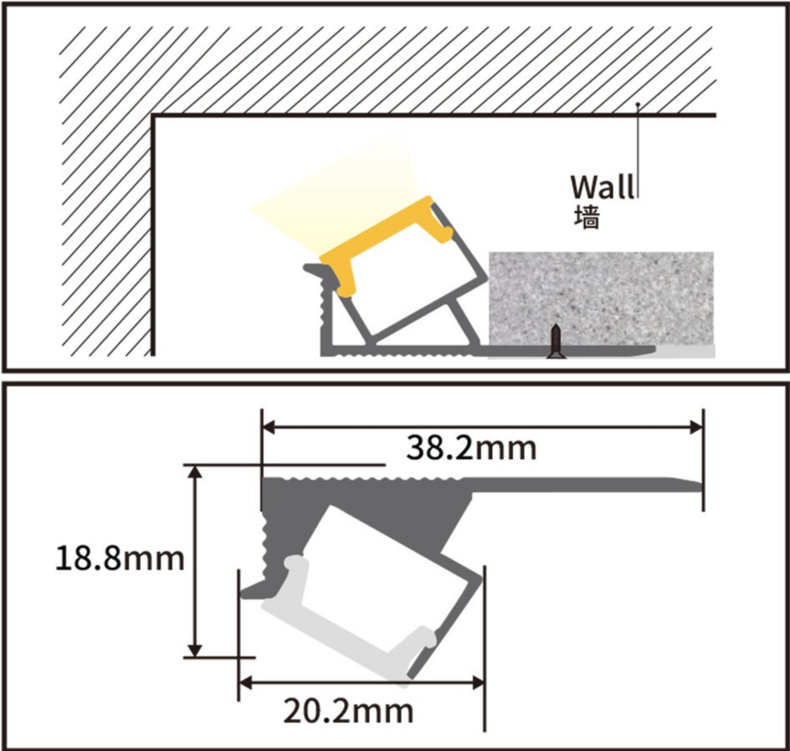
LFAPSL-XWL-38.2X18.8X20.2
