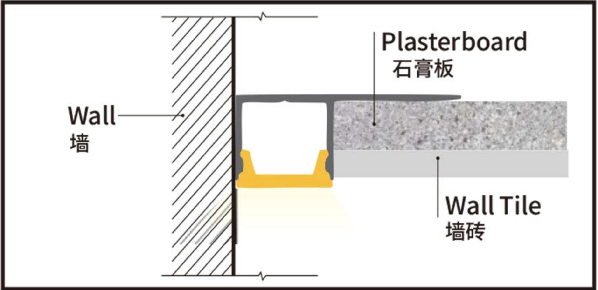
LFAPSL-SWL-34.4X14.1X15
