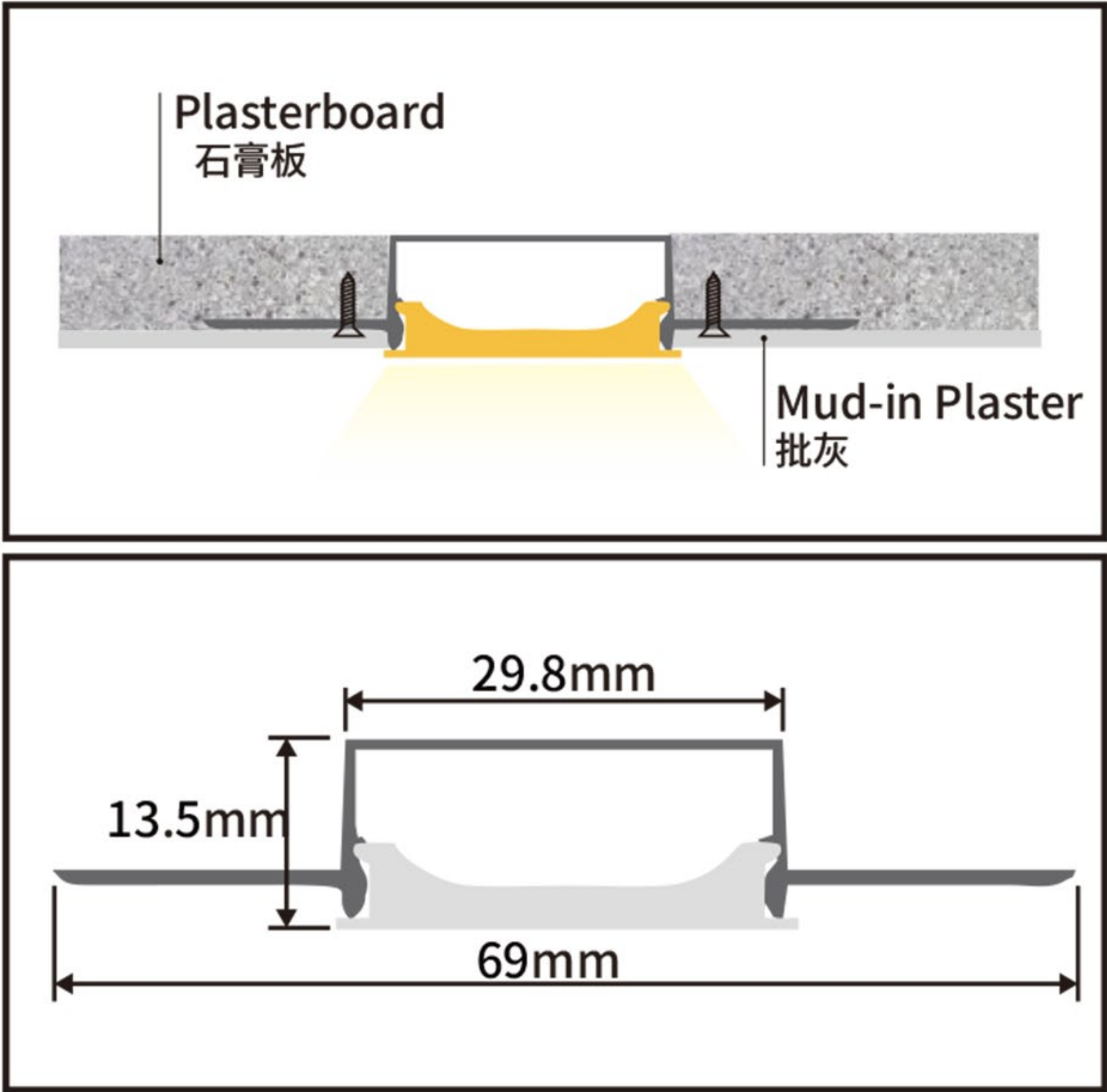
LFAPSL-DW-69X13.5X29.8
