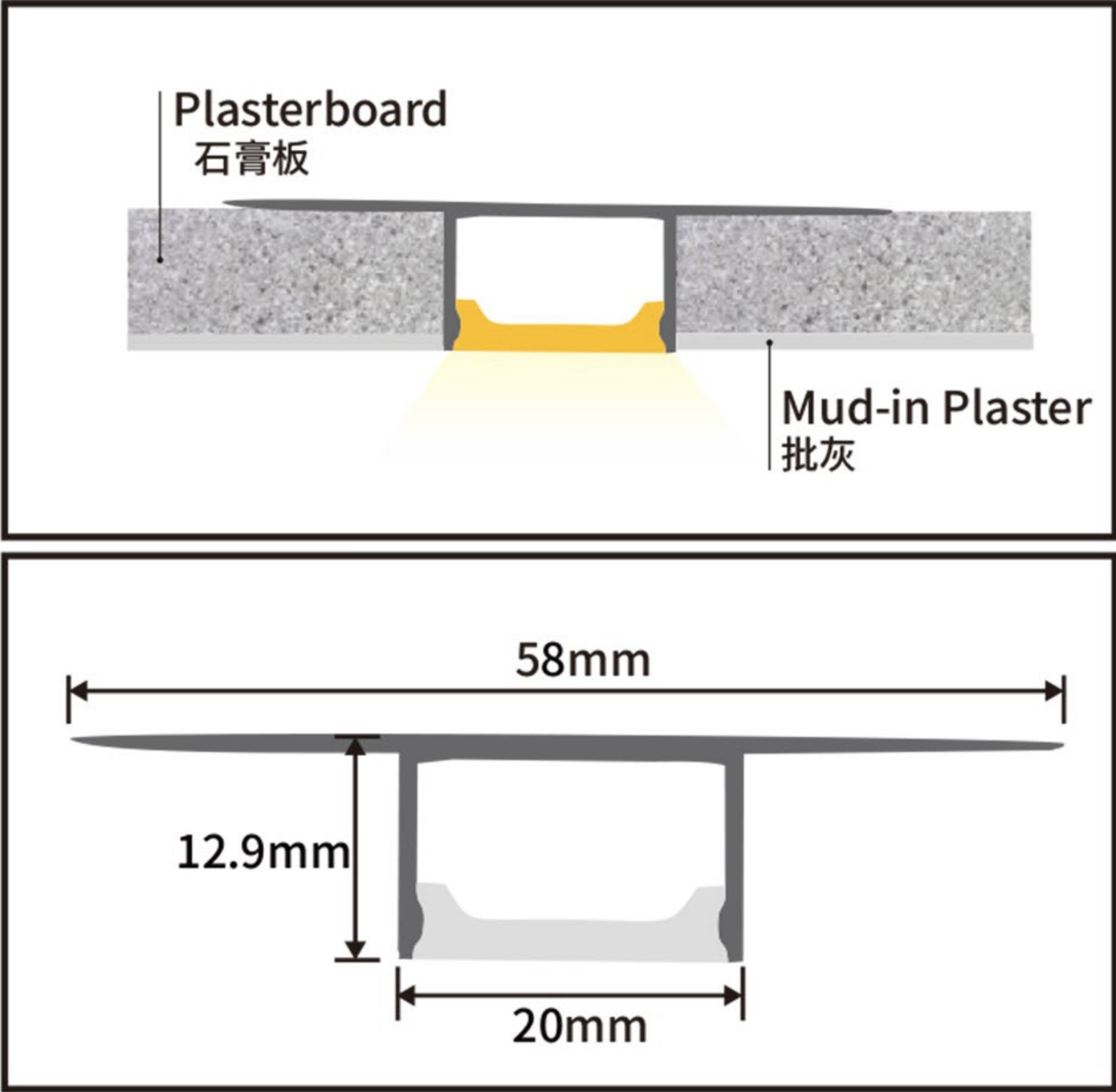
LFAPSL-DW-58X12.9X20
